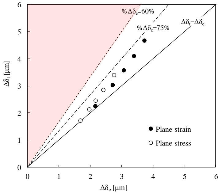
Figure 8. Effect of stress state on the relation between the elastic and total CTOD (AA2050-T8; MT160; R=0.1 ; a_0=5, 10, 15, 20, 25 mm).
