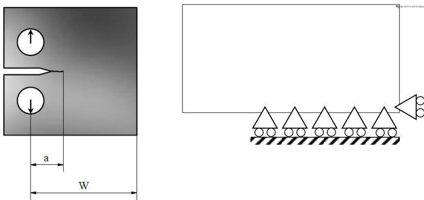
Figure 3. CT specimen (a) Main dimensions. (b) Boundary conditions.
