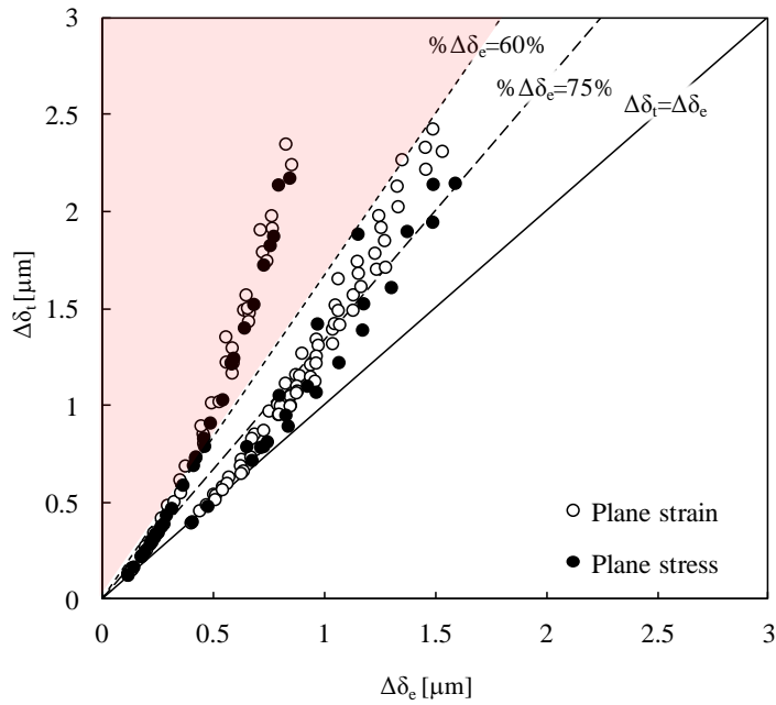
Figure 6. Representation of \Delta\delta_i as a function of \Delta\delta_e .
