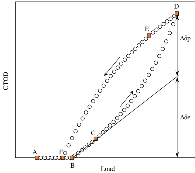
Figure 4. Typical plot of CTOD versus applied load.
