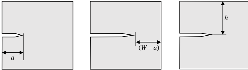
Figure 2. Situations where the LEFM is not valid, according ASTM E647 (CT and MT specimens).
