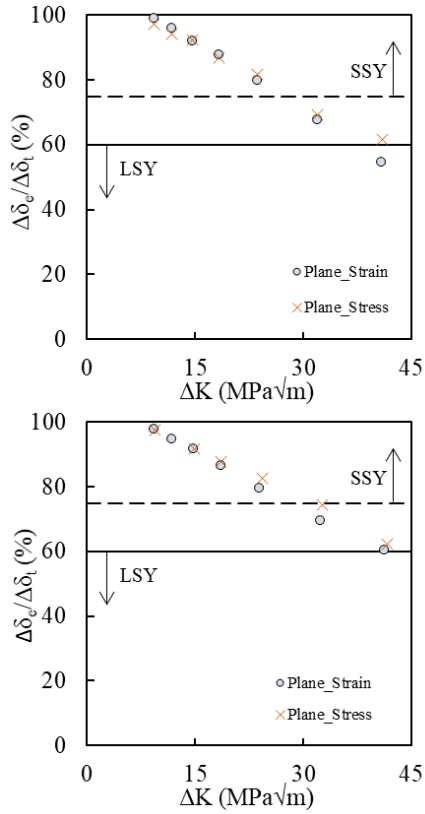
Figure 10. The effect of crack length and stress state on the transition from SSY to LSY for Ti6Al4V: CT36; R=0.05 ; a_0=7, 10, 13, 16, 19, 22 and 24 mm). (a) HIP manufacturing process; (b) Heat treatment to reduce the residual stresses.
