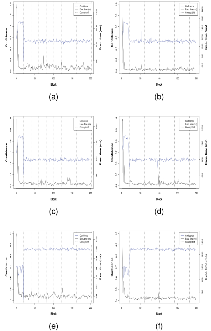
Fig. 5. Confidence and execution time performance of FEPDS on different datasets with concept drift. (a), (c), (e) Datasets with an abrupt drift. (b), (d), (f) Datasets with a gradual drift.
