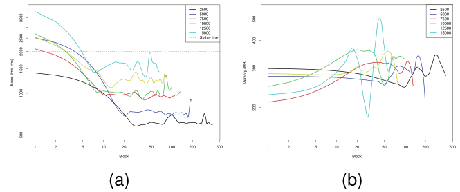
Fig. 6. Scalability analysis for the AG-cl-I data stream with respect to different data block size. (a) Processing time. (b) Memory consumption.
