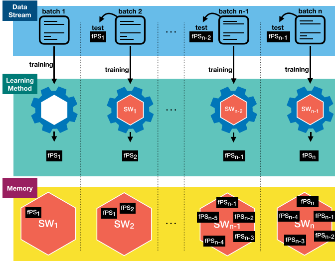
Fig. 4. General working schema of the FEPDS algorithm.
