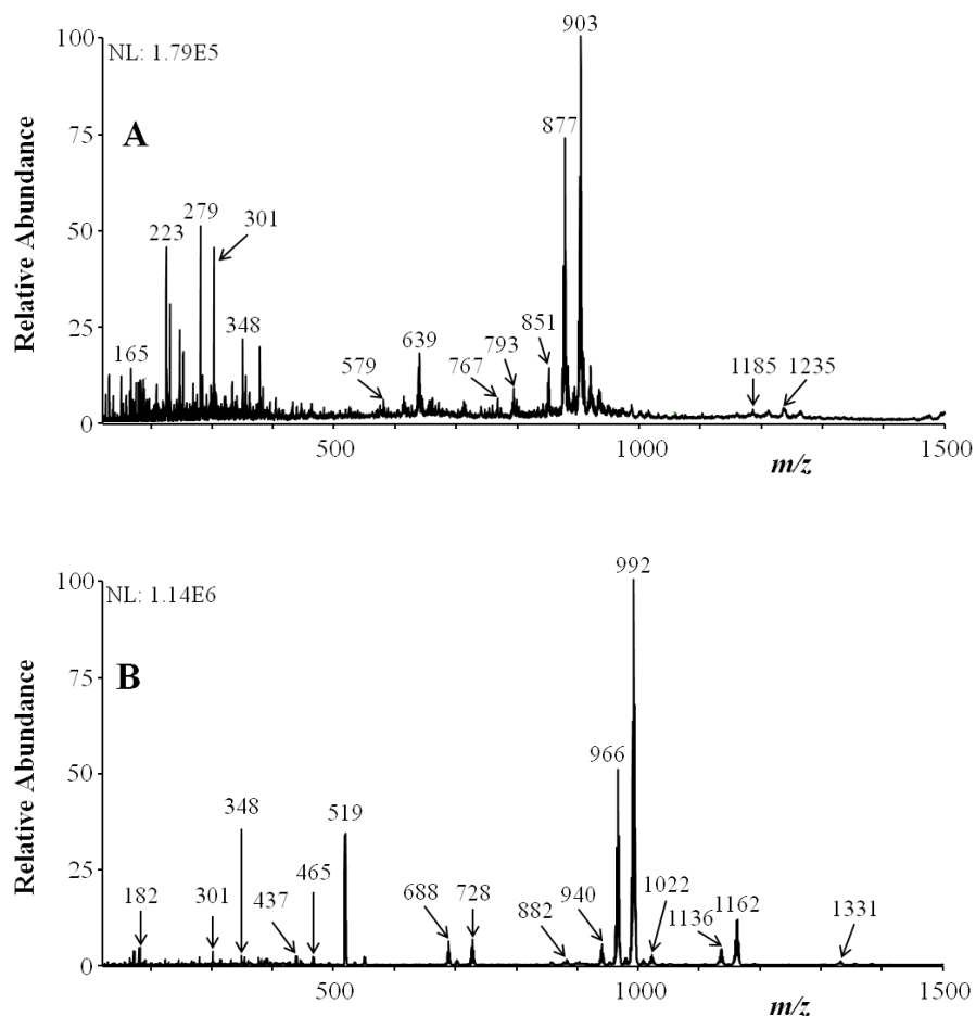
Figure 5. Paperspray mass spectra obtained in positive ion mode ( m/z range 120-1500) of an extra virgin olive oil diluted 1:1000 in isopropanol (A), and via silver adduct formation with 25 mM of \text{AgNO}_3 (B). For more details of MS acquisition conditions, see section 2.3.
