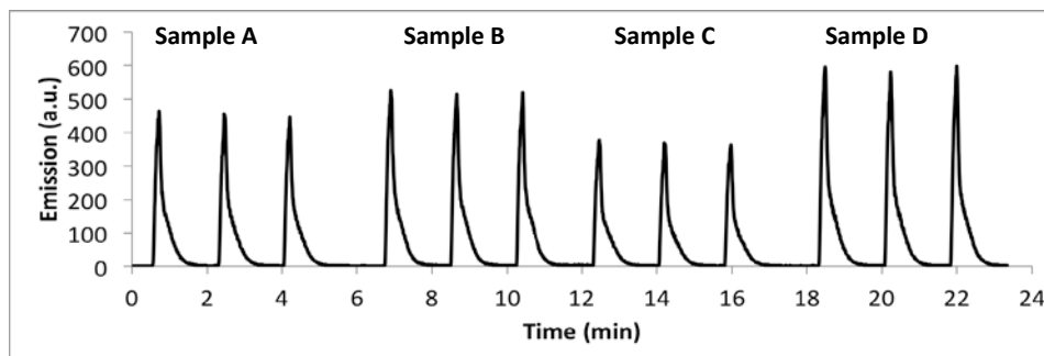
Figure 7. a) Profile diagram of calibration line. b) Typical signal profile corresponding to triplicate measures of four different EVOO samples.
