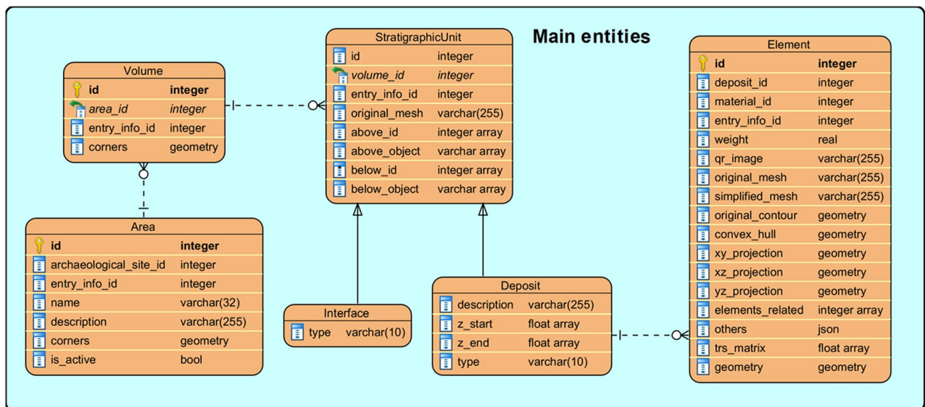
Fig. 4 Main data entities stored in the database
