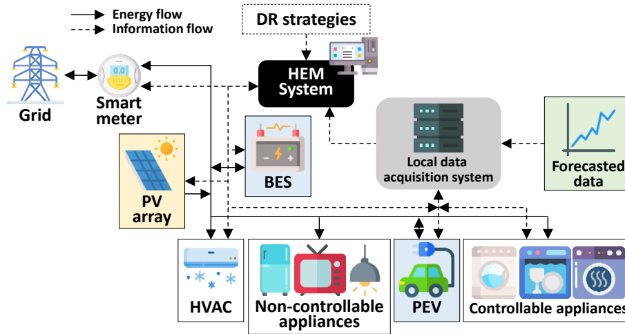
Fig. 2 Schematic representation of the analyzed prosumer environment
