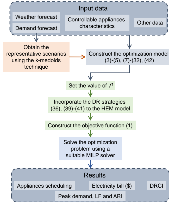
Fig. 4 Flowchart of the proposed HEM solution incorporating DR strategies
